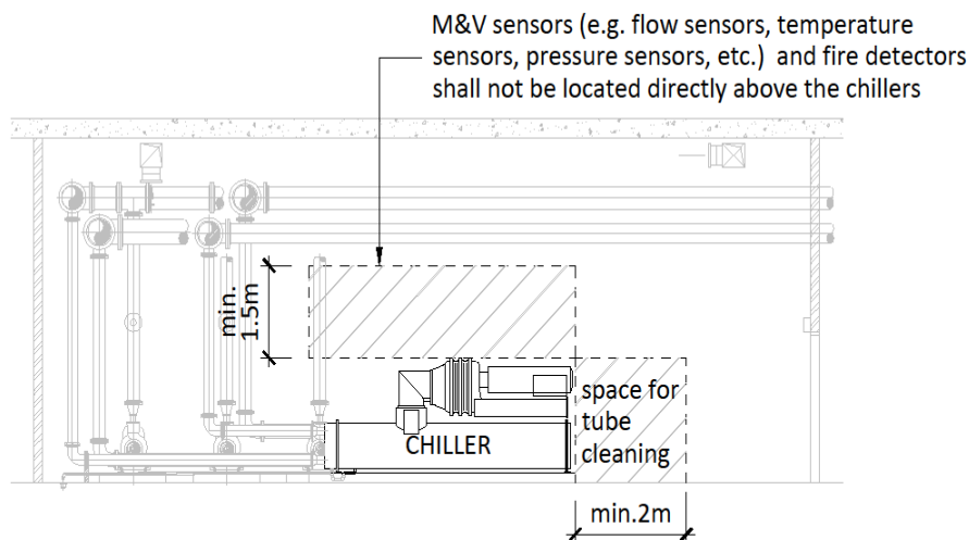
Figure 06-2 – Head room requirements for the chillers
