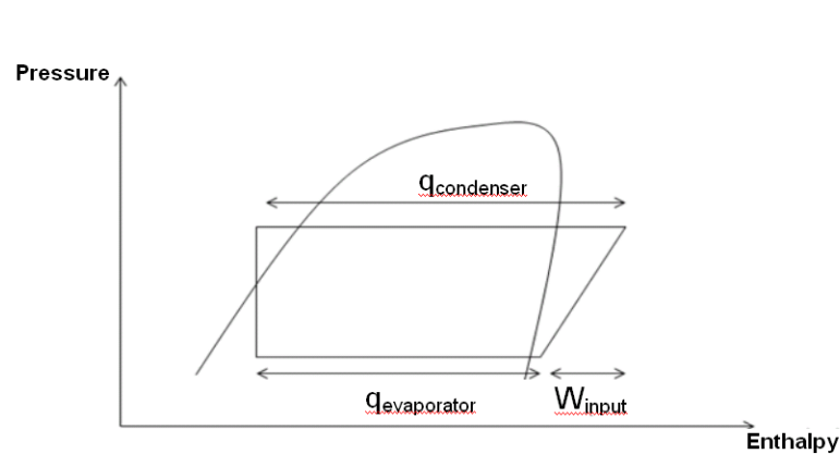
Pressure Enthalpy Chart
