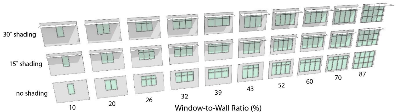
Illustration of the facade geometric parameters of various WWR and Shading provision with the respective OOA
