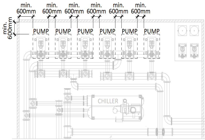
Figure A3 – Access space for the pump systems
